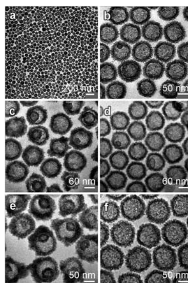
Figure 3. Single- and double-shelled \text{Cu}_2\text{S} hollow spheres: a) prepared with \text{Cu}(\text{NO}_3)_2/\text{CH}_4\text{N}_2\text{S} = 2:1 at 200/215 °C, and b)–f) prepared with \text{Cu}_2\text{O}:\text{Na}_2\text{S} = 1:1.5, 1:2, 1:3, 1:4, \text{ and } 1:5 , respectively, at room temperature (Supporting Information, Sections S1, S3).
